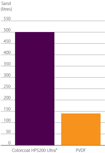
Figure 11. Abrasion resistance comparison (ASTM D968:2001)
