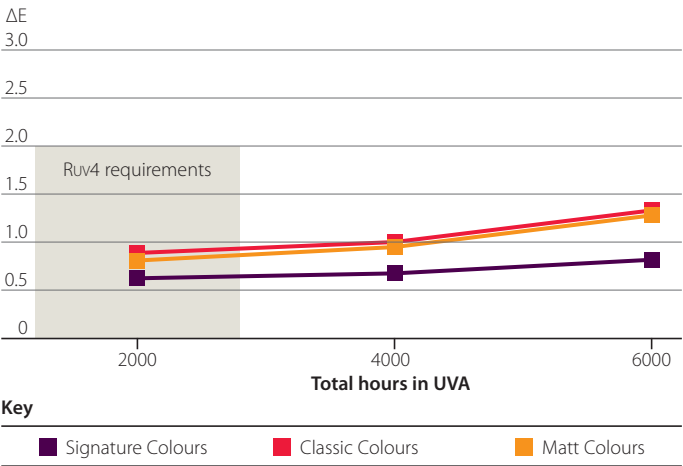
Figure 26. ΔE for Colorcoat HPS200 Ultra® in UVA
