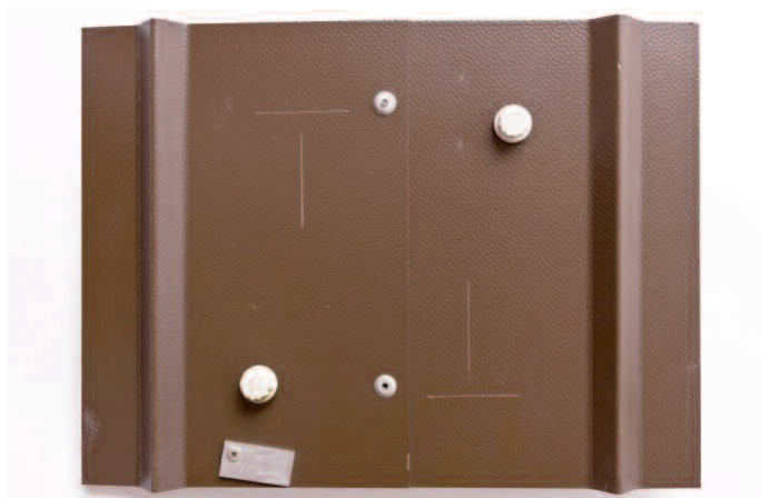
Figure 16. Colorcoat HPS200® with Galvalloy® metallic coating – 6 years exposure at coastal weathering site at Rye, England.
