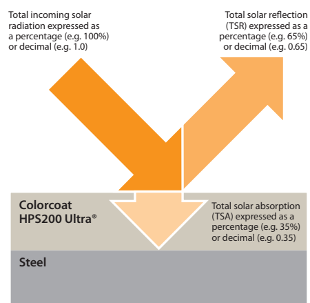
Figure 32. Solar reflectivity
