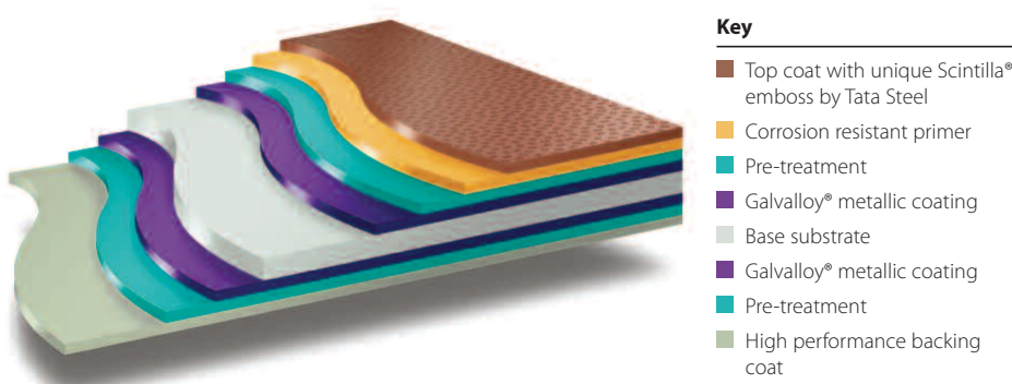
Figure 1. Colorcoat HPS200 Ultra® layers illustration
