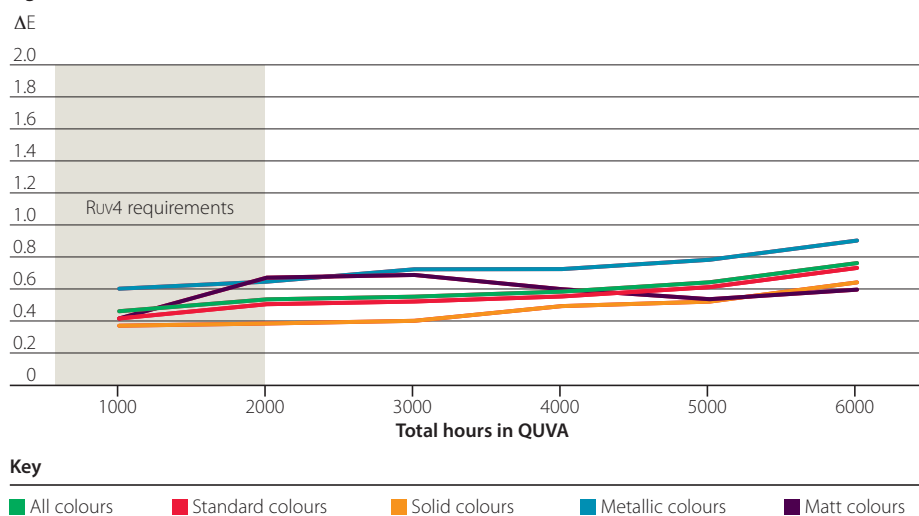
Figure 21. ΔE for Colorcoat Prisma® in QUVA
