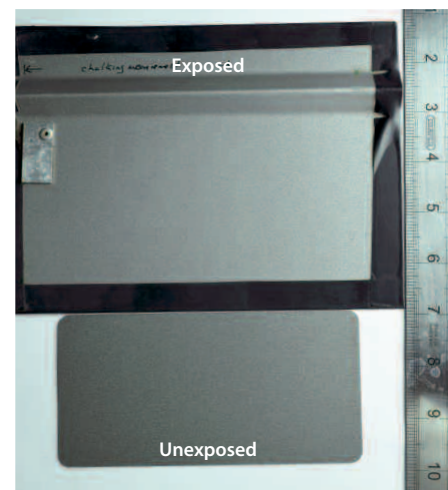
Figure 26. Colorcoat Prisma® Orion after 5 years exposure.
