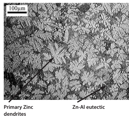
Figure 4. Typical Galvalloy® microstructure
