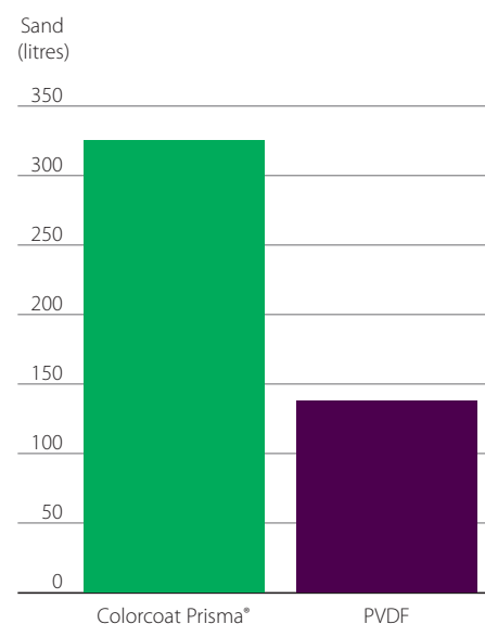
Figure 11. Abrasion resistance comparison (ASTM D968:2001)
