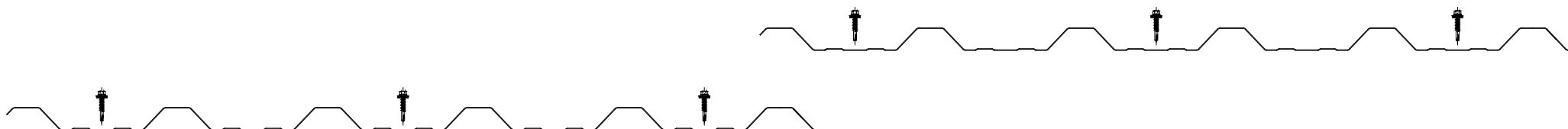
Fastener Pattern for : Intermediate purlin locations. Fix each side of sidelap and mid sheet, min 15mm diameter washers: 3No. fasteners per panel,
