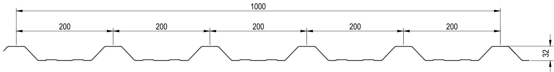
32/1000/200 Roof Profile
