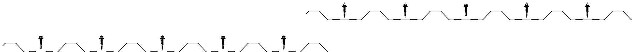
Fastener Pattern for : End Laps, Ridge and Eaves purlins. Fix through each trough, min 15mm diameter washers: 5No. fasteners per panel
